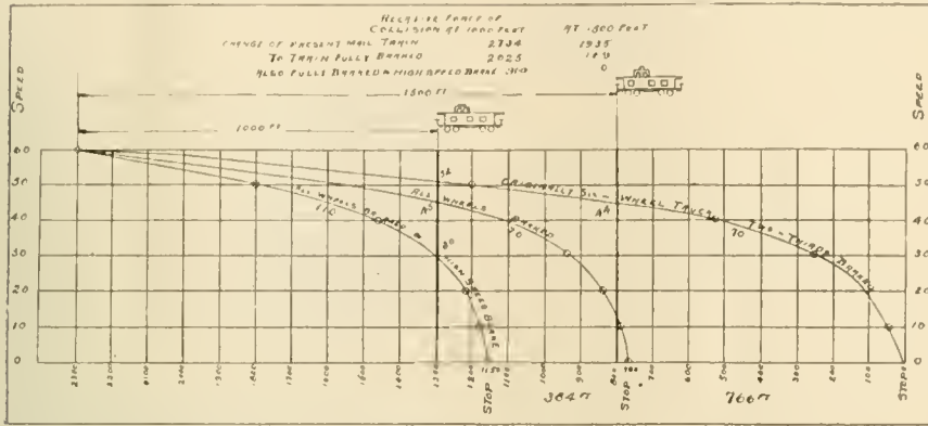
GRAPHIC COMPARISON OF STOPS MADE WITH LOW PRESSURE BRAKES AND HIGH SPEED BRAKES.
